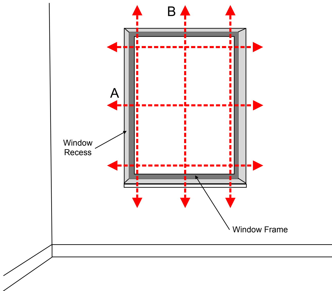
Blind Measurement for Outside Recess Diagram 2
